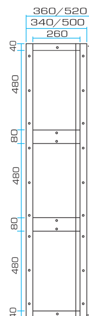
AS 1013
