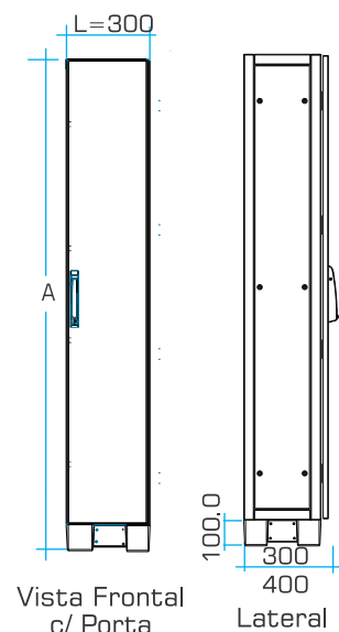
Coluna auxiliar
